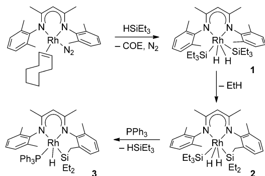
Scheme 2. Formation and rearrangement of 1 .
