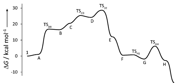
Figure 2. Calculated free-energy profile (b-p/TZVP) for the conversion of 1 to 2 via the path shown in Scheme 3.
