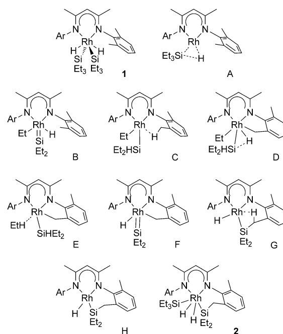
Scheme 3. Proposed intermediates for conversion of 1 to 2 .
